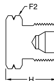
Blank Plug CGA 350
