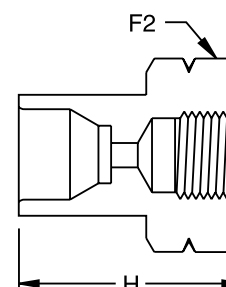
NPT Female CGA 350
