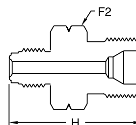
Vac Male CGA 350
