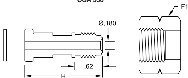
VacuSeal Male CGA 330
