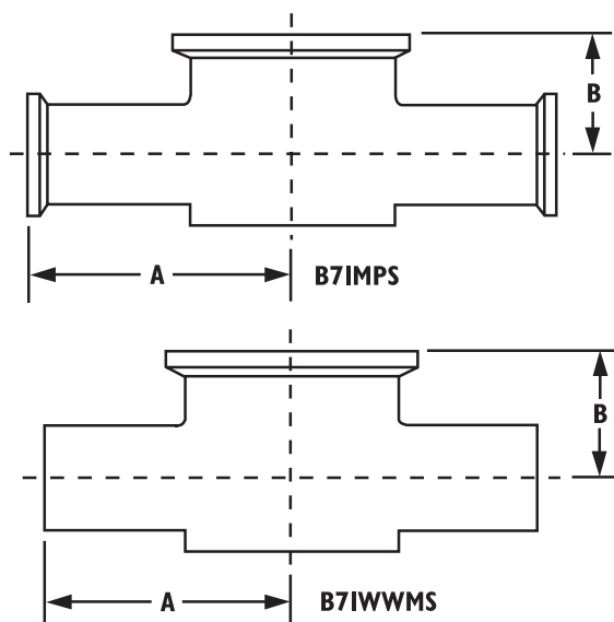
B7IMPS – Clamp Instrument Tee (TABLE DT-29)
