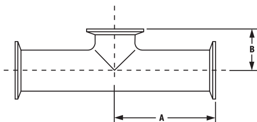
B7RMPS – Reducing Short Outlet (TABLE DT-20)
