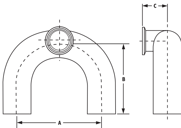
B2UMPSOA – Side Outlet Drain
