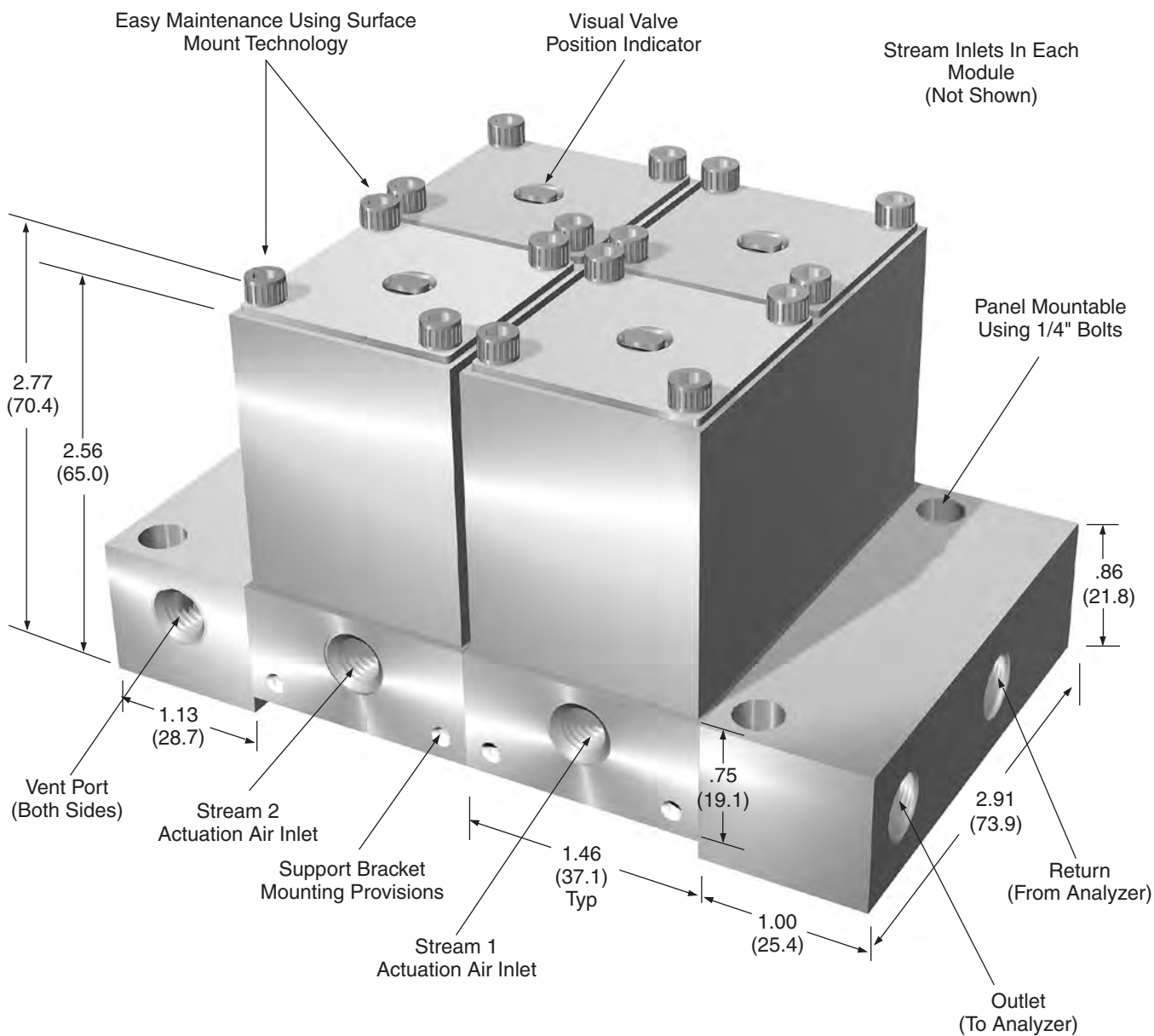
Factory Assembled Two Module Stream Switching System See How to Order – Page 8
