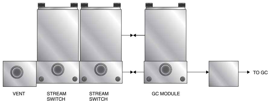
Example Shown: Two streams with GC Module
